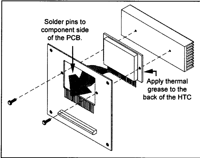
Assembly of HTCPCB evaluation (99-840008)
