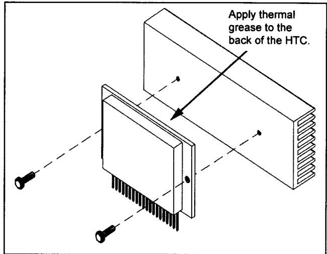
Assembly of HTC heatsink (99-850000)
